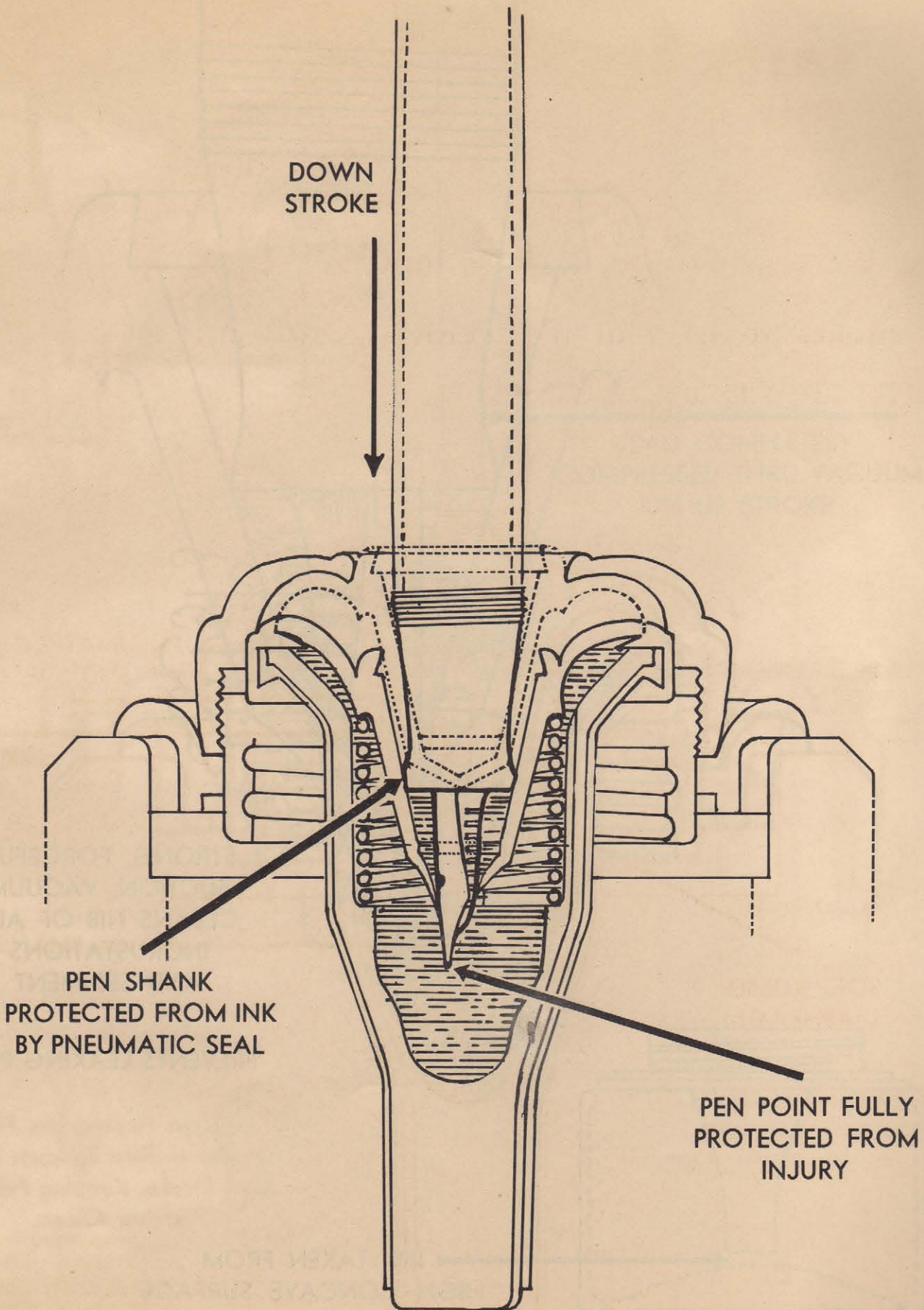
SECOND — Compression Stroke (Gently Pressed Down About 1/4 Inch)
